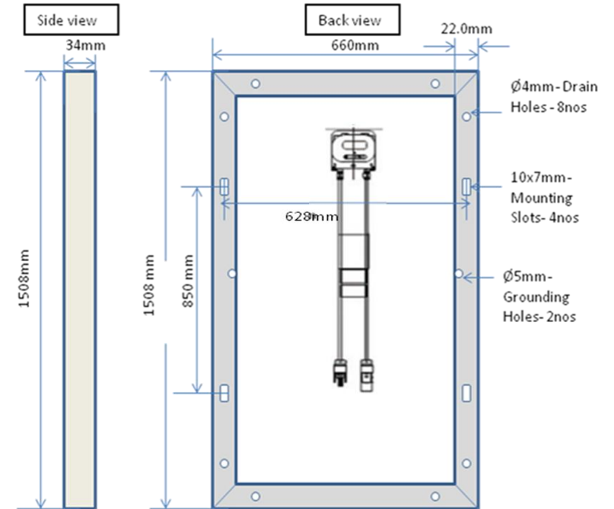
Mechanical Dimension:
